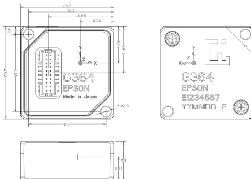
Outline Dimensions (millimeters)
